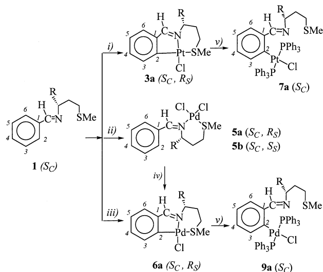
Scheme 1. R = CO 2 Me. i) cis -[PtCl 2 (dmsO) 2 ] in refluxing methanol. ii) Na 2 [PdCl 4 ] in methanol at room temperature. iii) Na 2 [PdCl 4 ] and NaAcO in refluxing methanol. iv) NaAcO in refluxing methanol. v) PPh 3 in CDCl 3 at room temperature
