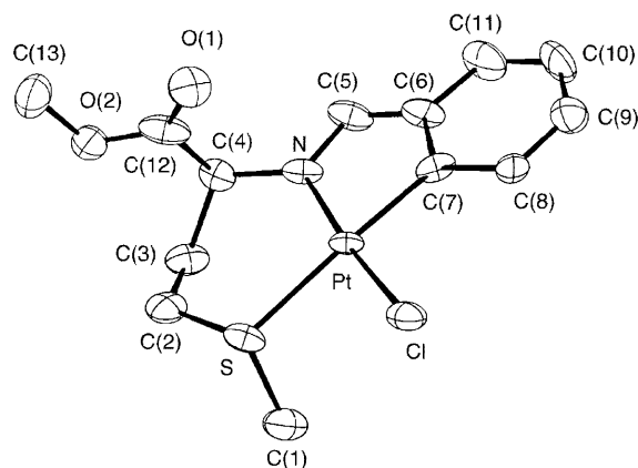
Figure 1. ORTEP diagram of the crystal structure of (S_C,R_S)-(+)-[\text{Pt}\{\text{C}_6\text{H}_4-\text{CH}=\text{N}-\text{CH}(\text{CO}_2\text{Me})-\text{CH}_2-\text{CH}_2-\text{SMe}\}\text{Cl}] ( 3a ). Selected bond lengths [in Å]: Pt–N, 1.984(11); Pt–S, 2.349(3); Pt–Cl, 2.308(4); Pt–C(7), 1.954(14); N–C(5), 1.954(14). Selected bond angles [in deg.]: C(7)–Pt–Cl, 94.0(4); N–Pt–S, 99.2(3); Cl–Pt–S, 85.84(13); N–Pt–Cl, 174.8(3); Pt–N–C(5), 114.9(11); N–C(5)–C(6) 119.6(16)
